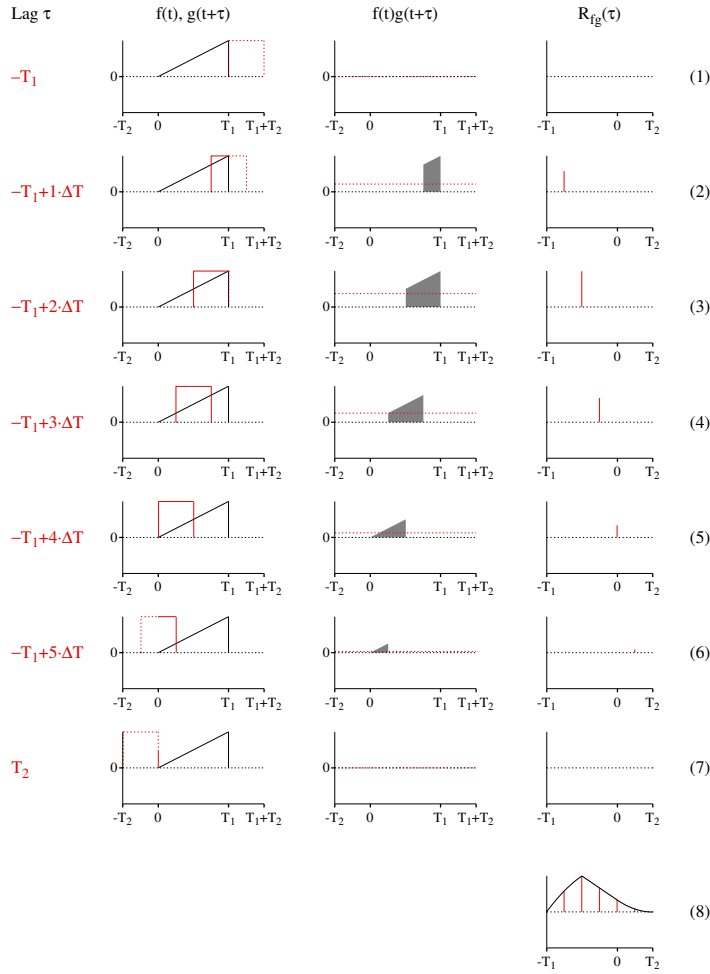
Figure A.24.: Calculation of the cross-correlations of two simple functions f(t) and g(t) for different values of lag time \tau . Column 1: lag time \tau , where \Delta T = (T_1 + T_2)/6 . Column 2: f(t) in black and g(t+\tau) in red. Column 3: product function h(t) = f(t)g(t+\tau) with red dotted line showing its average value. Column 4: the cross-correlation value at the lag position, where the vertical axis has been expanded for clearer display. The bottom panel shows the accumulation of the seven cross-correlation values in red together with the complete cross-correlation function in black.
