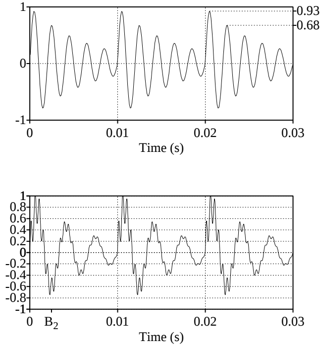
Figure 13.2.: Top: The oscillogram of two sound segment with one formant (top: F = 500 Hz with B = 50 Hz) and two formants (bottom: F_1 = 300 Hz with B_1 = 50 Hz and F_2 = 2100 Hz with B_2 = 100 Hz). For both sounds the F_0 equals 100 Hz.
