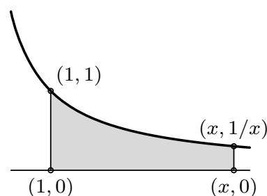
Fig. 6. Natural logarithm.
