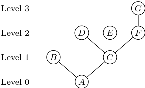
Fig. 15. A tree.
