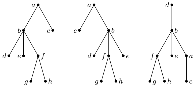
Fig. 35. Three tree structures.
