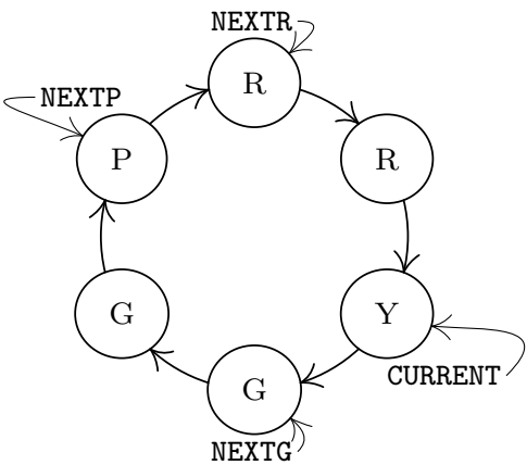
Fig. 26. Input and output from the same circle.
