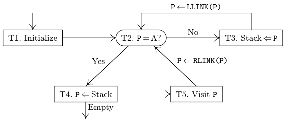
Fig. 23. Algorithm T for inorder traversal.
