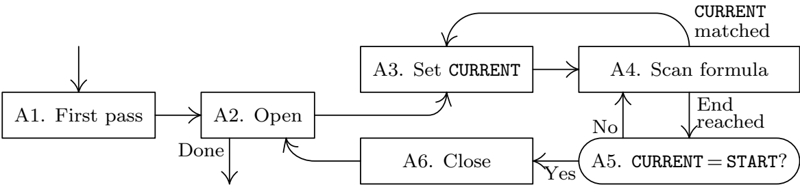
Fig. 20. Algorithm A for multiplying permutations.
