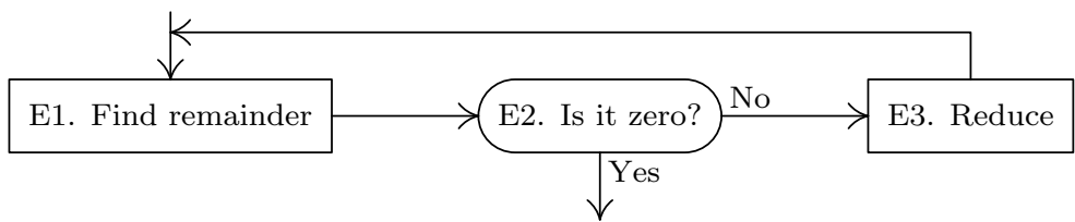
Fig. 1. Flow chart for Algorithm E.
