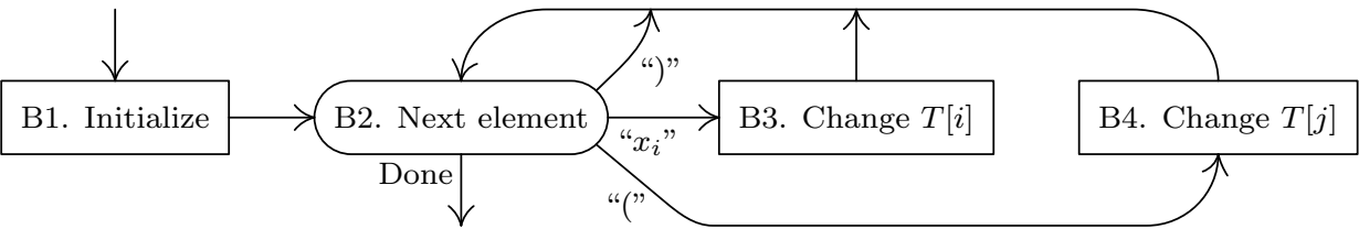
Fig. 21. Algorithm B for multiplying permutations.
