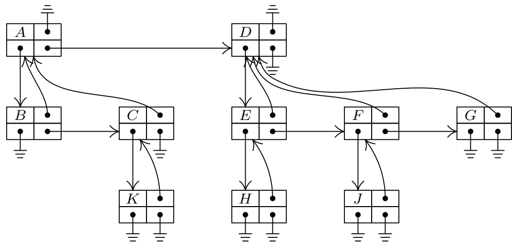
Fig. 26. A triply linked tree.
