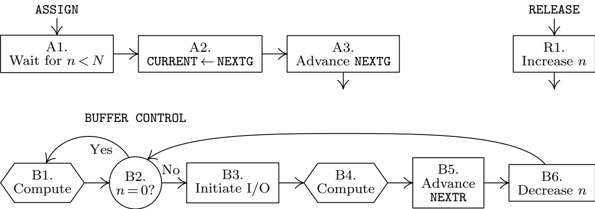
Fig. 25. Algorithms for multiple buffering.
