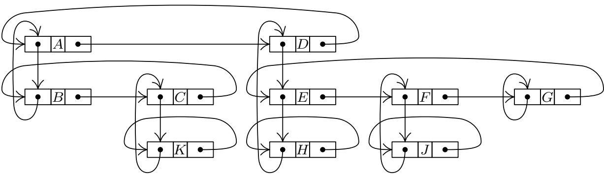
Fig. 27. A ring structure.
