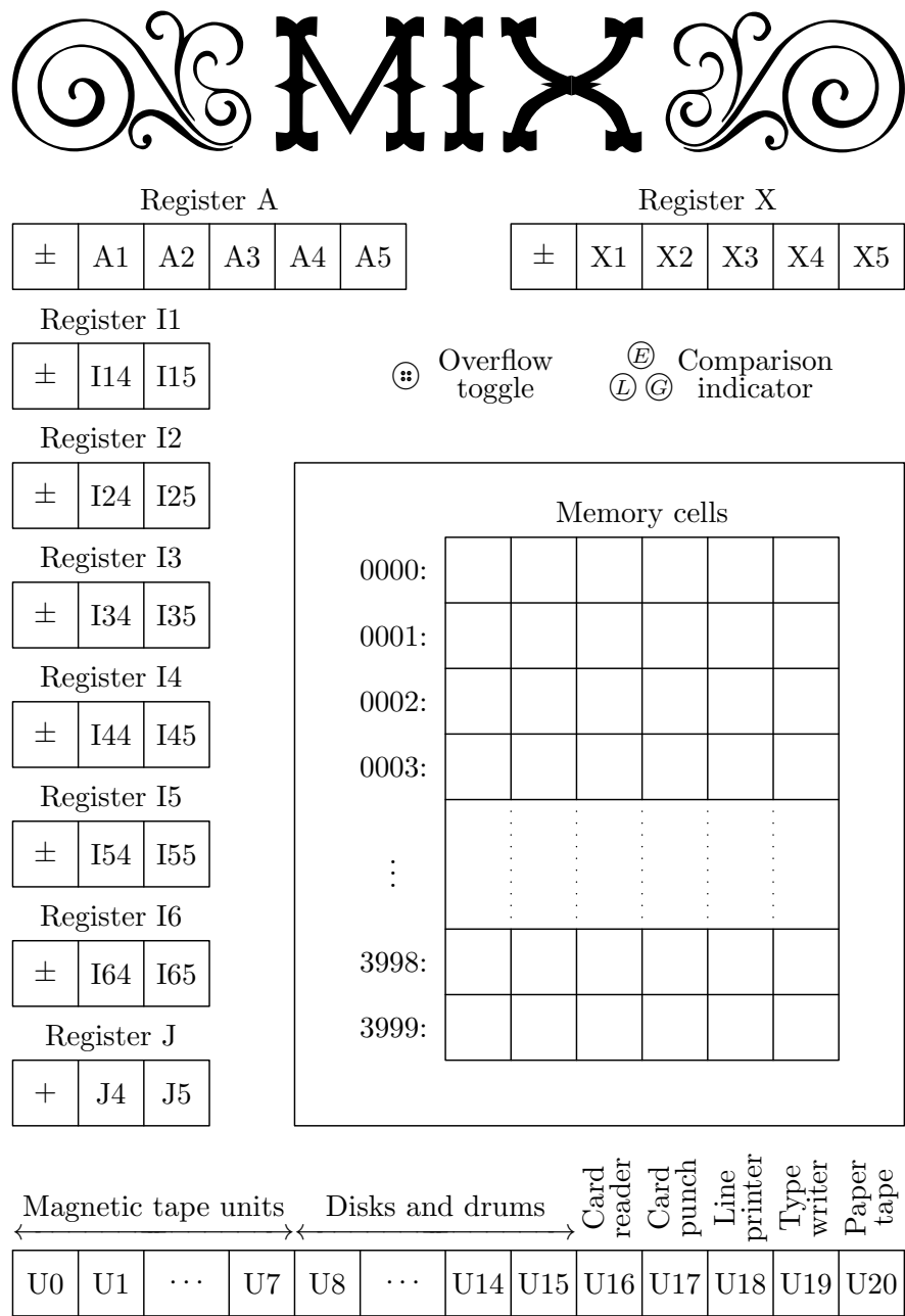
Fig. 13. The MIX computer.
