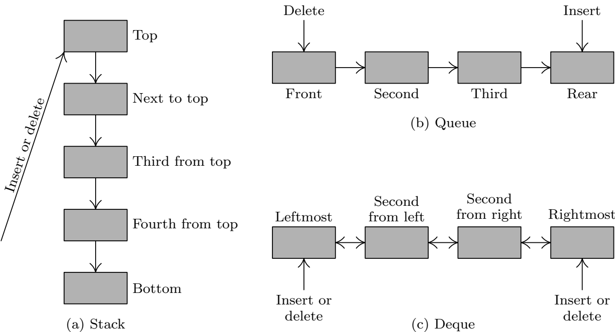
Fig. 3. Three important classes of linear lists.
