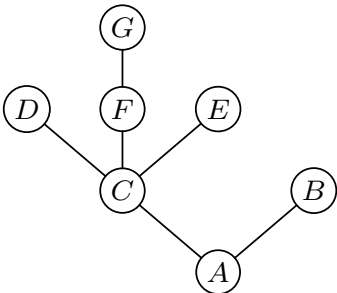
Fig. 16. Another tree.
