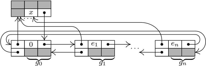
(c) Polynomial = g_0 + g_1x^{e_1} + g_2x^{e_2} + \dots + g_nx^{e_n}
