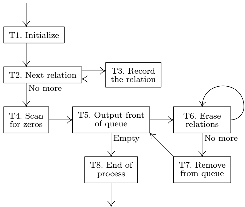
Fig. 9. Topological sorting.
