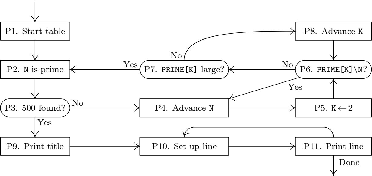
Fig. 14. Algorithm P.
