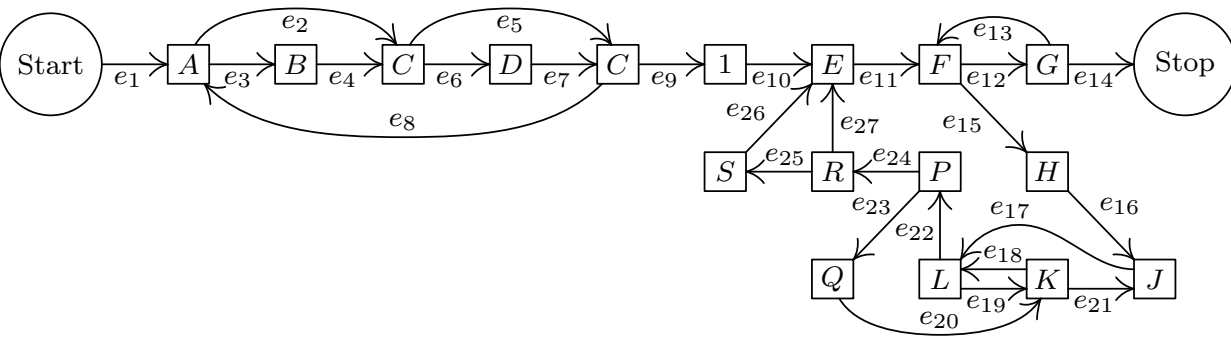
Fig. 31. Abstracted flow chart of Program 1.3.3A.
