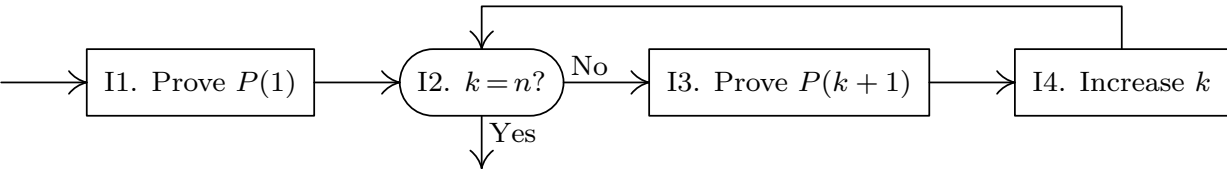
Fig. 2. Algorithm I: Mathematical induction.
