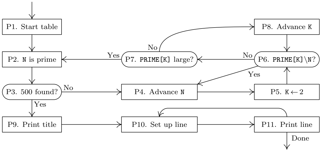
Fig. 14. Algorithm P.
