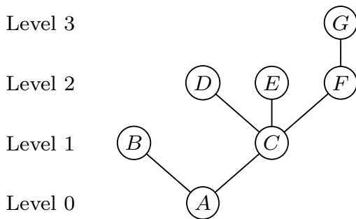
Fig. 15. A tree.
