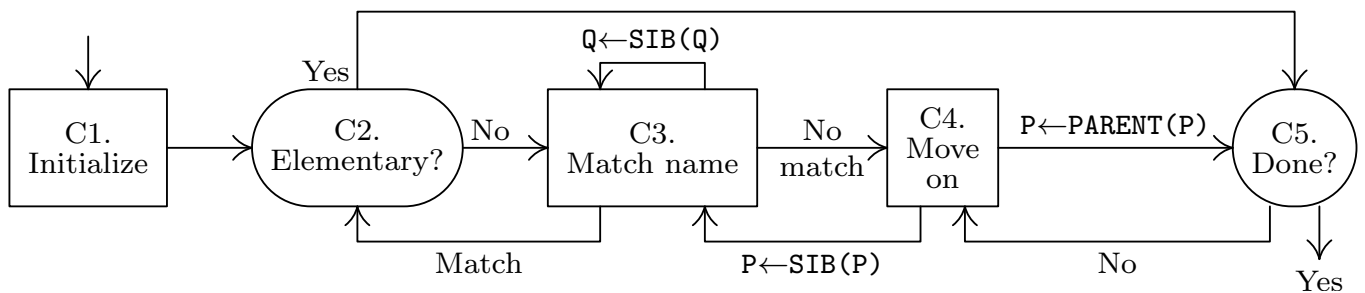
Fig. 41. Algorithm for “MOVE CORRESPONDING”.
