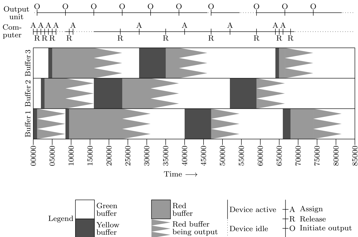
Fig. 27. Output with three buffers (see exercise 9).
