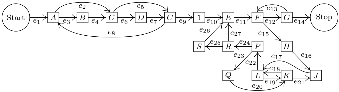
Fig. 31. Abstracted flow chart of Program 1.3.3A.
