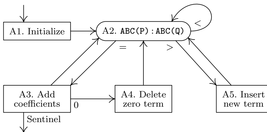
Fig. 10. Addition of polynomials.
