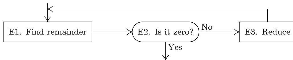
Fig. 1. Flow chart for Algorithm E.
