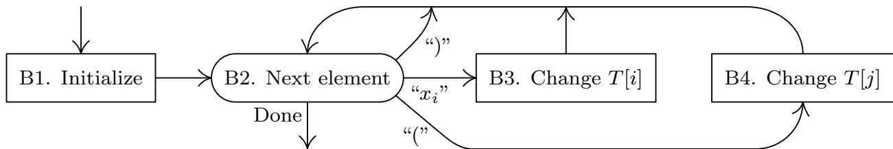
Fig. 21. Algorithm B for multiplying permutations.
