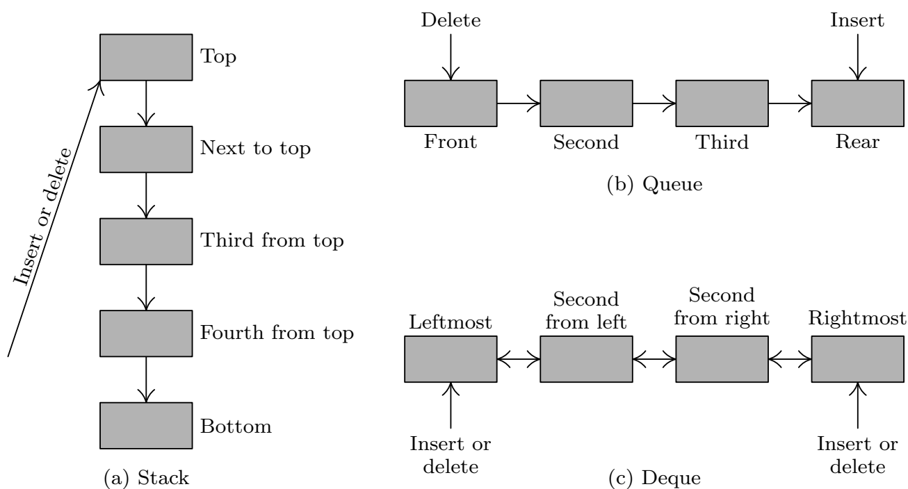
Fig. 3. Three important classes of linear lists.
