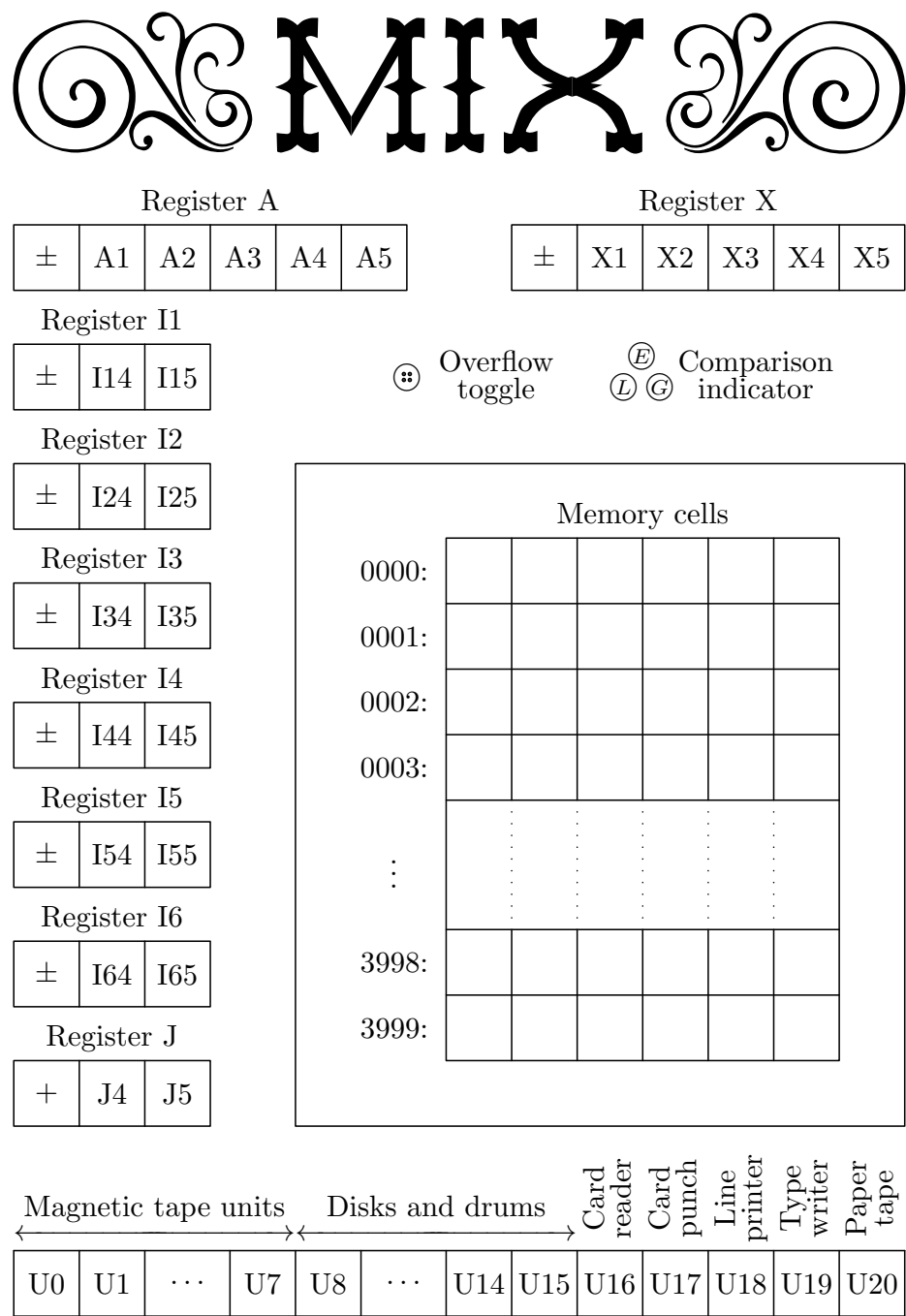
Fig. 13. The MIX computer.
