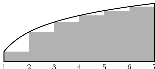
Fig. 12. Comparing a sum with an integral.
