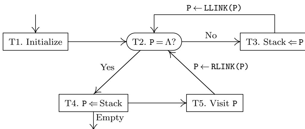
Fig. 23. Algorithm T for inorder traversal.
