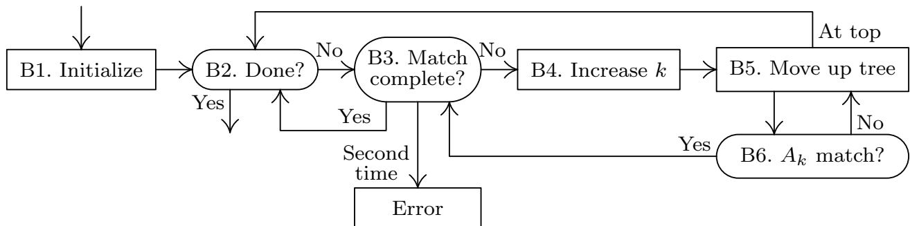
Fig. 40. Algorithm for checking a COBOL reference.
