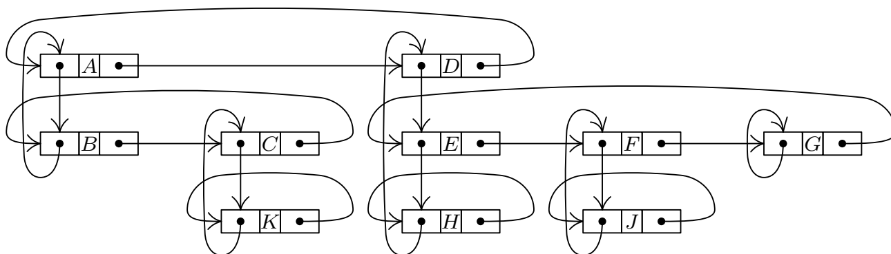
Fig. 27. A ring structure.
