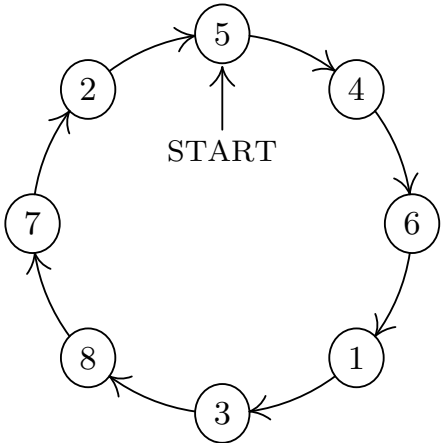
Fig. 17. Josephus's problem, n = 8 , m = 4 .
