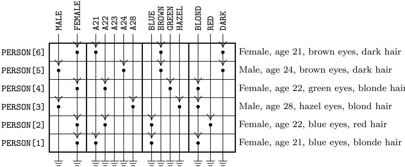
Fig. 13. Each node in four different lists.
