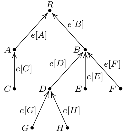
Fig. 34. An oriented tree.
