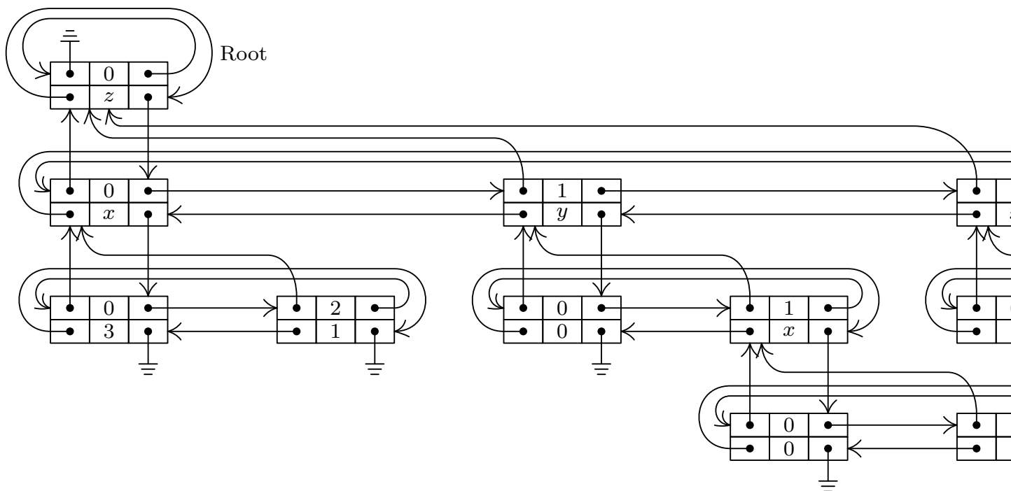
Fig. 28. Representation of polynomials using four-directional links. Shaded areas of nodes indicate the context considered.
