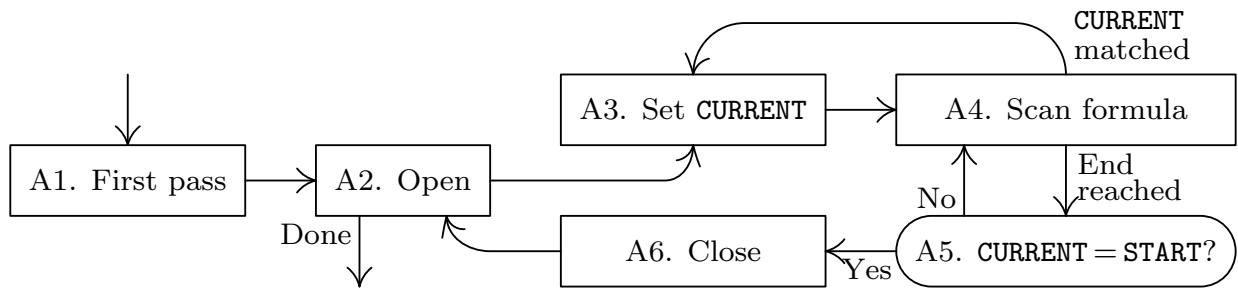
Fig. 20. Algorithm A for multiplying permutations.
