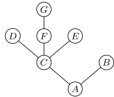
Fig. 16. Another tree.
