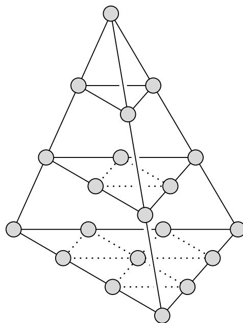
Fig. 8. Geometric interpretation of \binom{n+2}{3} , n = 4 .
