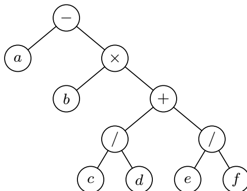
Fig. 21. Tree representation of formula (2).
