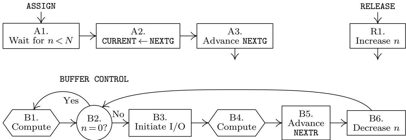
Fig. 25. Algorithms for multiple buffering.
