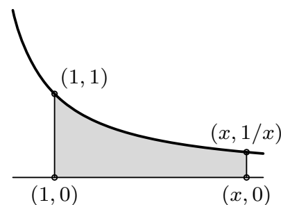
Fig. 6. Natural logarithm.
