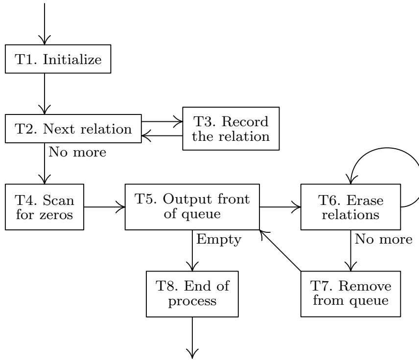
Fig. 9. Topological sorting.
