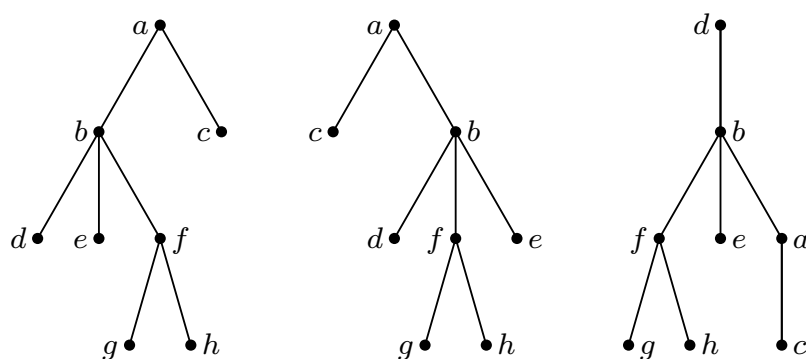
Fig. 35. Three tree structures.
