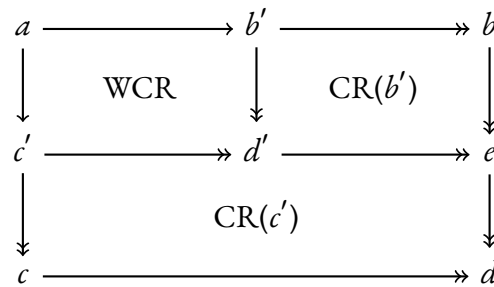
Figure 3: An illustration of the proof of Newman’s Lemma by well-founded induction.
