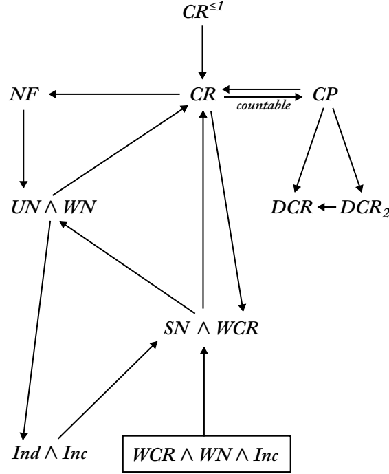
Figure 2: An overview of the interrelations between ARS properties that we have formalized. Note that there are implications which are true, but not shown in this figure (such as DCR \Rightarrow CR ), because they are not formalized in this work. Arrows pointing from or to a conjunction symbol refer to the entire conjunction; pointing from or to a conjunct refer only to that conjunct.
