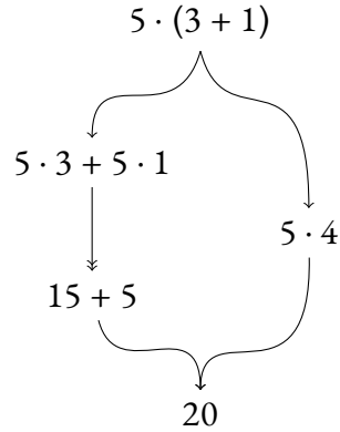
Figure 1: When simplifying arithmetic expressions, any diverging steps will converge again; the rewriting system we use to simplify arithmetic expressions is confluent .
