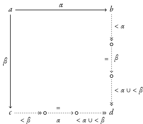
Figure 6: A decreasing elementary diagram.
