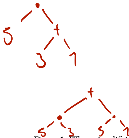
Figure 1: When simplifying arithmetic expressions, any diverging steps will converge again; the rewriting system we use to simplify arithmetic expressions is confluent .
